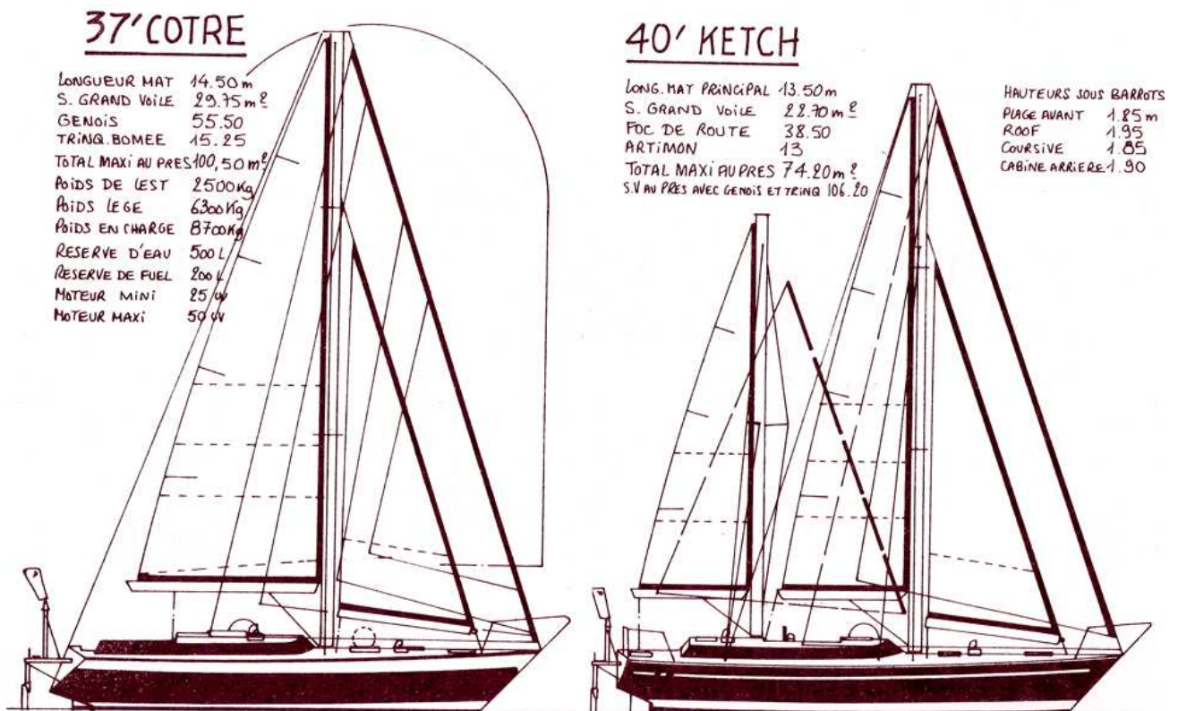
37/40- Polyester 11,80/12,50 m x 3,98 1974
