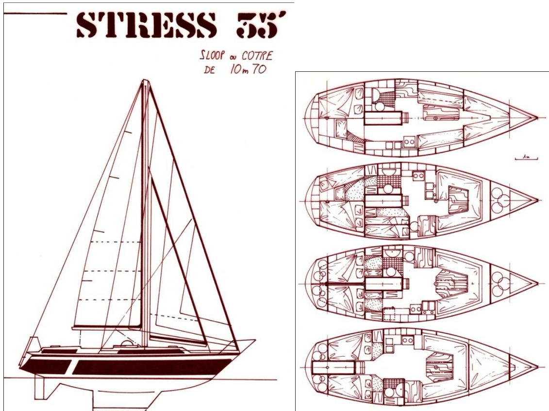
35' Polyester (Stress 35) 10,70 x 3,55 m 1973
