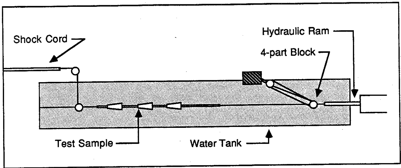
FIGURE 20. Fatigue Test Setup
