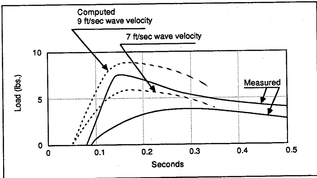
FIGURE 6. Drogue Loads
