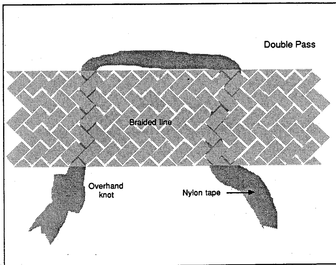
FIGURE 18. Splicing Methods
