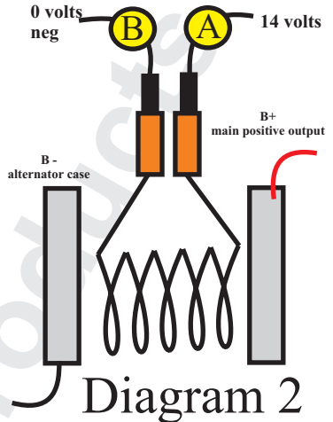
Basic alternator control: Diagram 2
