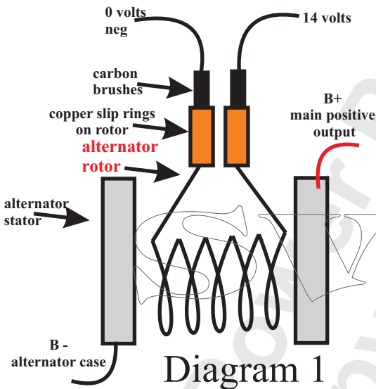
Basic generic alternator control system Diagram 1
